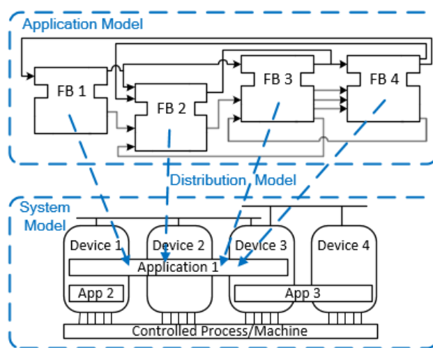
Fig. 1. Application, System and Distribution Model of IEC 61499
