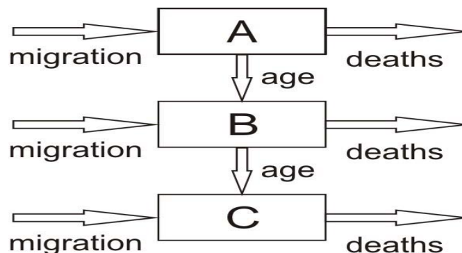
Figure 2. Scheme of age compartments, each compartment is changed through flows of migration and deaths, and people switch to the next compartment because of ageing
