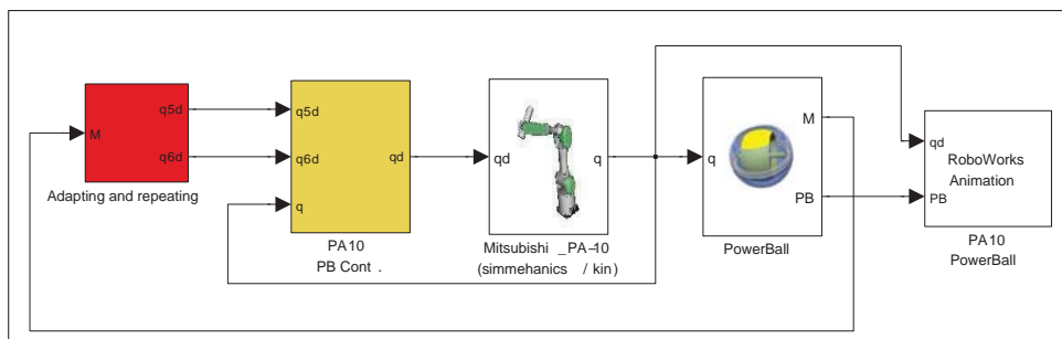
Figure 24: Power®Ball simulation: top level block scheme in Simulink and animation of the PA10 robot on Nomad platform and the Power®Ball
