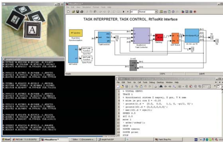
Figure 23: Vision based manipulation experiment: Robot is picking cube “A”
