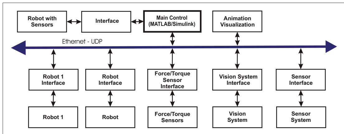
Figure 2: A functional block diagram of the robot integrated environment in Robotics Laboratory including the robot PA10, mobile platform Nomad XR 4000 and sensor systems
