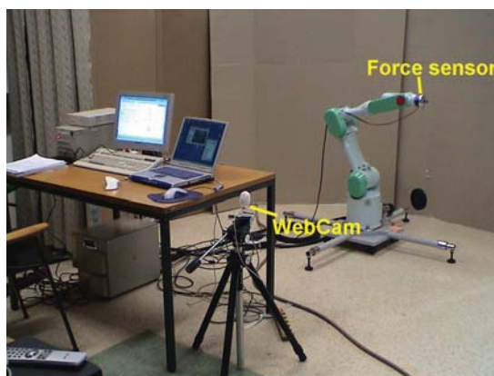
Figure 3: Experimental setup (Mitsubishi PA10, vision system and force sensor)
