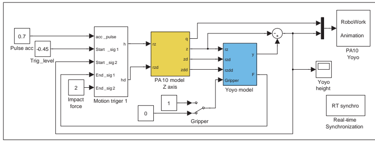
Figure 13: The case with kinematic PA10 robot model and external yo-yo simulator
