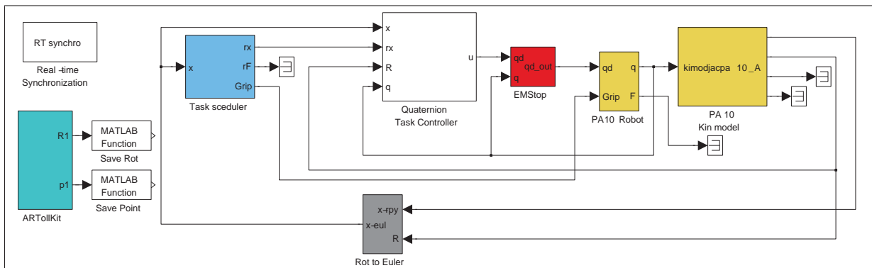
Figure 22: Vision based manipulation: Simulink block scheme
