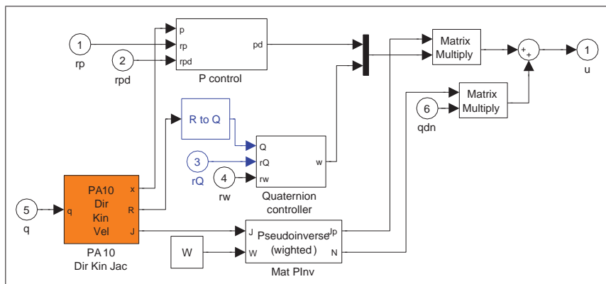
Figure 7: A block diagram representing the task space controller
