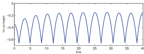
Figure 16: Swinging yo-yo motion - Simulation results
