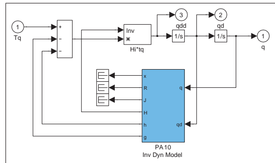
Figure 6: The dynamic model of the PA10 robot
