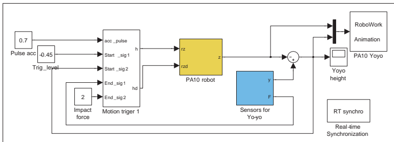
Figure 17: Hardware-in-the-loop simulation (real PA10 robot, force sensor and vision systems are in the simulation loop)
